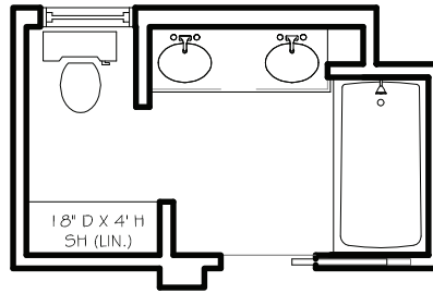
OPT. MBATH LAYOUT
